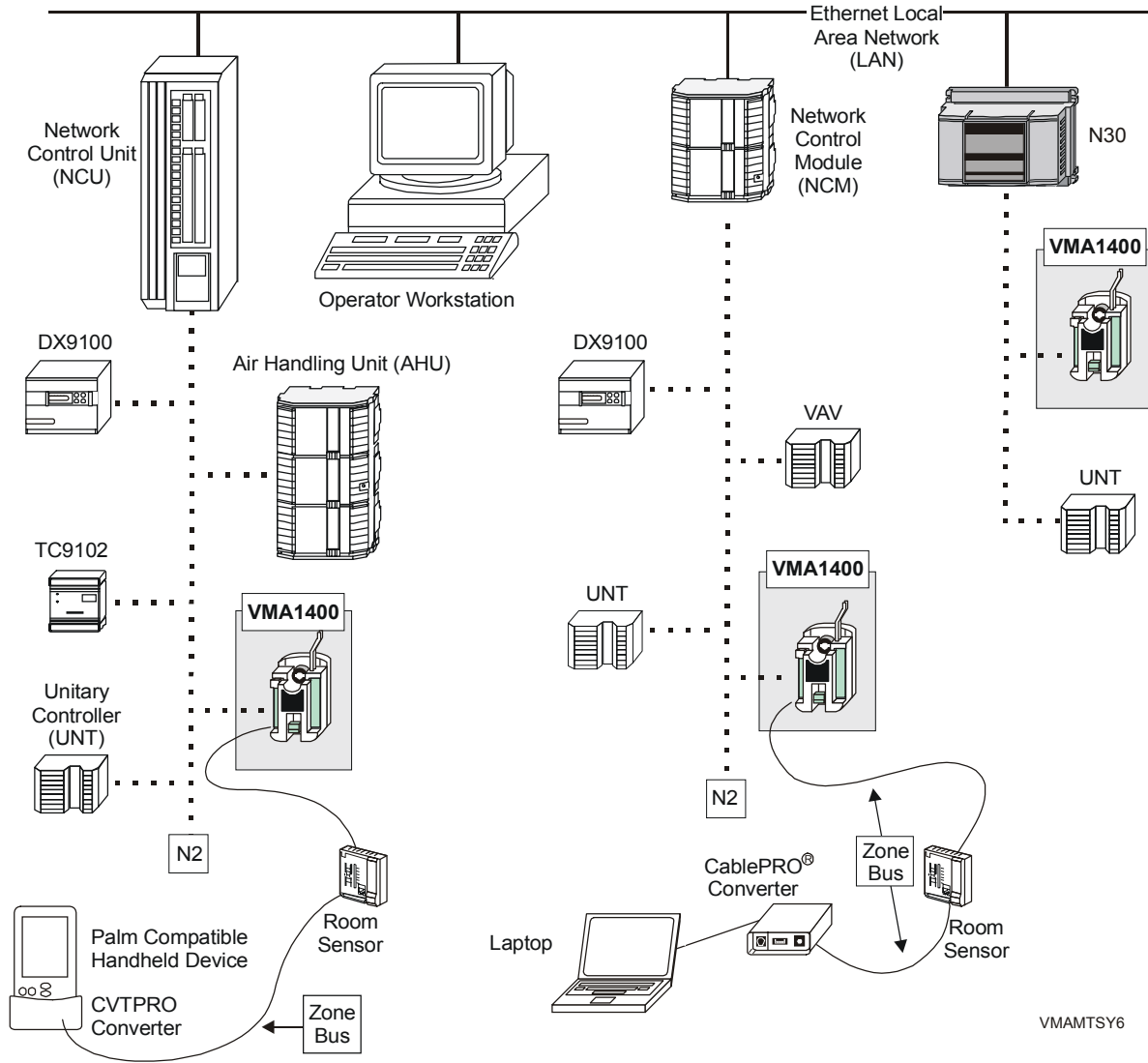
Figure 2: VMA in Metasys Network Diagram
